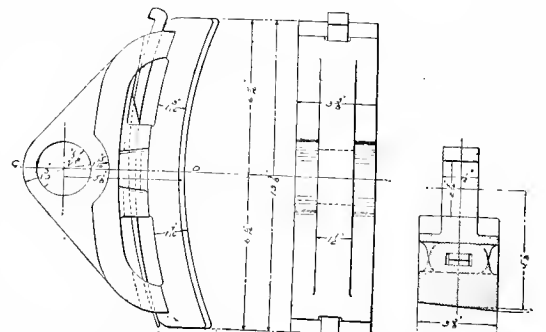
Figs. 1572-1574. Brake Head and Shoe.
